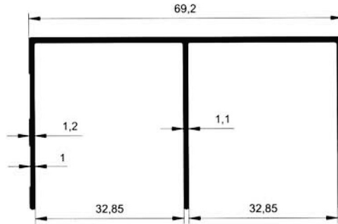
5805 0.551 kg/m
