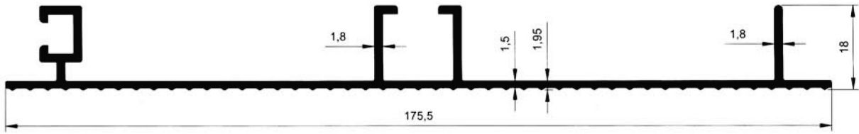
5656 BAZA 0.531 kg/m
