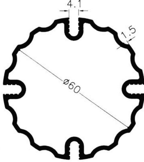
5273 1.030 Kg/m
