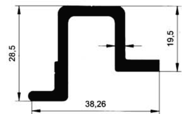
5573 0.692 kg/m
