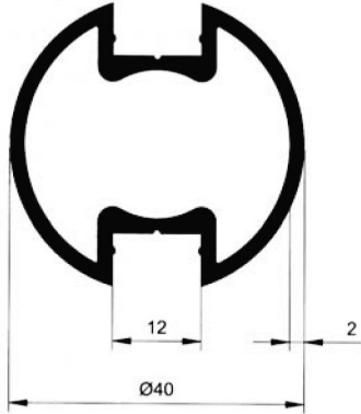
5366 0.845 kg/m
