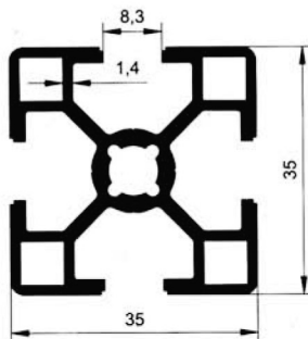
5570 0.967 kg/m
