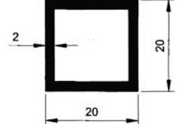
5481 0.390 kg/m
