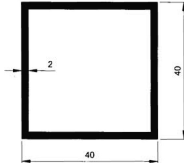
5487 0.821 kg/m
