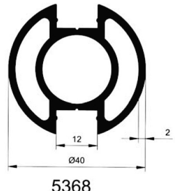
5368 1.084 kg/m
