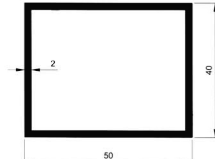
5488 0.932 kg/m
