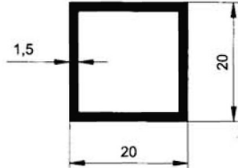
5786 0.301 kg/m
