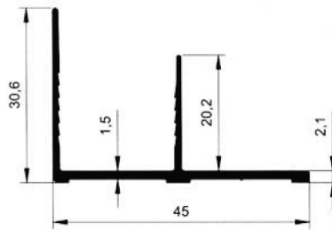
5764 0.339 kg/m
